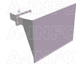
LB-650-15-C-7/16FSPO Standard Gain Horn Antenna 1.12-1.7GHz 15dB Gain 7/16(DIN) Female
